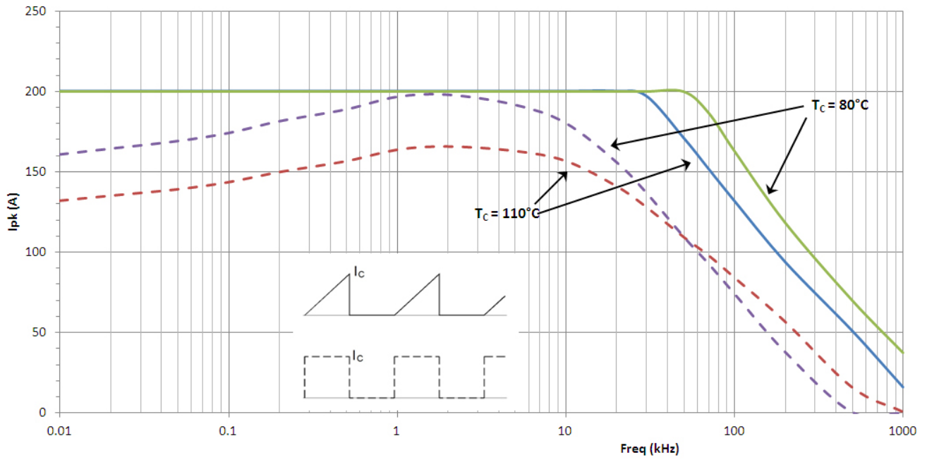
Figure 21. Collector Current vs. Switching Frequency
